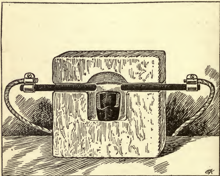
FIG. 11.—Moissan's electric furnace.
